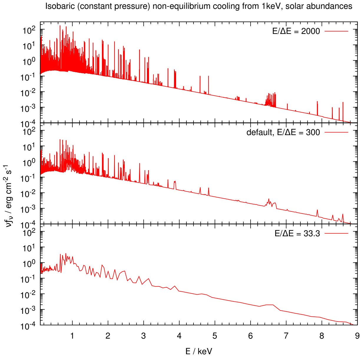
Figure 14.1: The X-ray spectrum of a unit-volume parcel of gas cooling under conditions of constant pressure (isobarically) from X-ray temperatures (1 keV), computed at three resolving powers. In the top panel, the resolving power is comparable the proposed Athena resolving power around 6 keV. In the bottom panel, the resolving power is comparable to the Chandra non-dispersive resolving power around 1 keV. In the middle panel, the resolving power is at the code default. This functionality is described in Chatzikos et al. (2015) .
