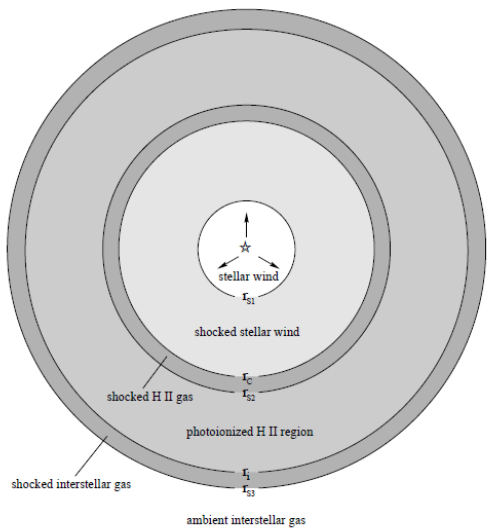
FIG. 1.—Schematic structure of an SWB: r_{s1} marks the position of the reverse shock, r_c the contact discontinuity, r_{s2} the forward shock of the stellar wind bubble, r_{i2} the ionization front, and r_{s3} the forward shock of the H II region expansion.
