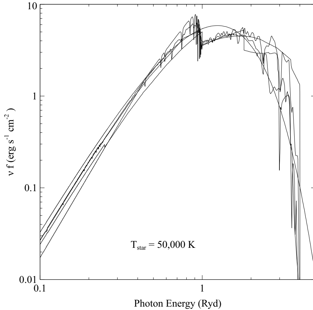
Figure 6.4: This figure shows the emergent radiation field predicted by five 5e4 \text{ K} stars included with the code. The smoothest is the blackbody, and the Kurucz (1991) and Rauch (1997) atmospheres show the most structure. stars
